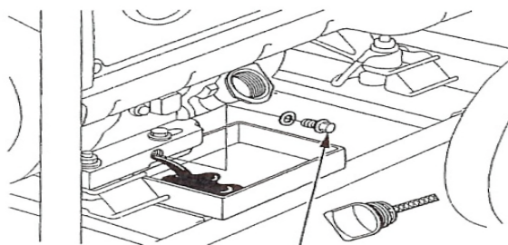
OIL DRAIN PLUG
